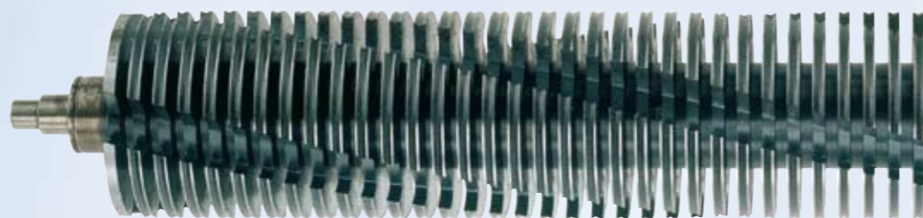
V-TEK by HSM The V-TEK groove of the cutting rollers is a ground-breaking development of HSM in terms of shredding equipment. The extremely efficient and high-precision cutting mechanism of the V-TEK groove ensures a considerably higher cutting capacity at at equivalent energy consumption.
